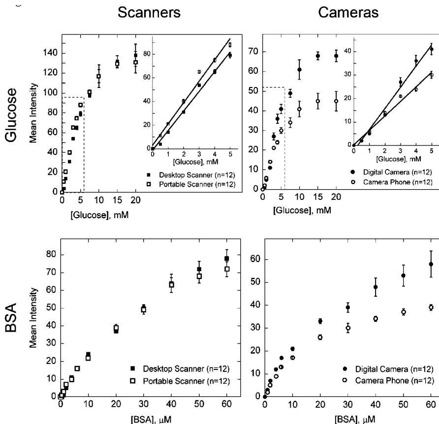
Figure 6. Analytical calibration plots for different concentrations of glucose and protein in artificial urine. The mean intensity for each data point was obtained from the histogram in AdobePhotoshop, as described in Figure 4. We measured concentrations of glucose between 0 and 20 mM. The protein assay was run using concentrations of BSA between 0 and 60 \mu\text{M} . The graphs contain data obtained using a desktop scanner (■), a portable scanner (□), a digital camera (●), and a camera phone with automatic focus (○); the inset shows the linear region of the data in greater detail. Each datum is the mean of twelve assays; error bars represent the relative standard deviations of these measurements. For the glucose assay, the linear region of the data was fit with a line (shown in the inset); the slope ( m ), intercept ( b ), and R^2 value for each line are as follows: desktop scanner ( m = 16.6 , b = -1.54 , R^2 = 0.991 ), portable scanner ( m = 18.0 , b = 2.95 , R^2 = 0.986 ), digital camera ( m = 8.96 , b = -2.12 , R^2 = 0.983 ), and camera phone ( m = 6.17 , b = 0.186 , R^2 = 0.986 ). The protein data was fit with a quadratic equation; the quadratic coefficient ( a ), the linear coefficient ( b ), the constant coefficient ( c ), and the R^2 value for each curve are as follows: desktop scanner ( a = -0.015 , b = 2.15 , c = 0.955 , R^2 = 0.996 ), portable scanner ( a = -0.017 , b = 2.20 , c = 1.36 , R^2 = 0.998 ), digital camera ( a = -0.012 , b = 1.62 , c = 3.81 , R^2 = 0.987 ), and camera phone ( a = -0.012 , b = 1.29 , c = 3.36 , R^2 = 0.986 ).
