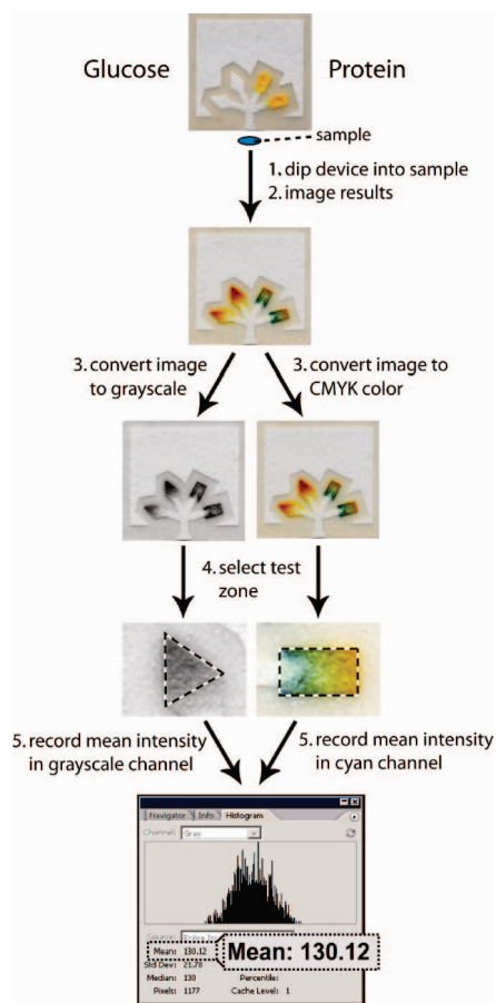
Figure 5. Procedure for quantifying the levels of glucose and protein in urine using image editing software (we used AdobePhotoshop). For the glucose assay, we converted the scanned or photographed digital images to 8-bit grayscale and selected the appropriate test zone of the device. For the protein assay, we converted the image to CMYK color and measured the intensity of cyan. The mean pixel values within the test zones correlate with the concentration of the analyte.
