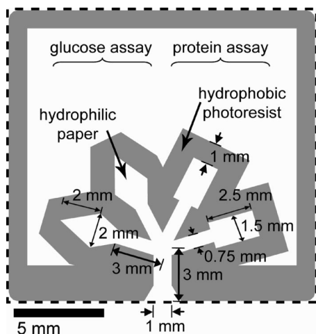
Figure 2. Design of a prototype paper-based microfluidic device that quantifies two analytes in urine simultaneously. The central channel at the bottom of the device wicks the sample into the four separate test zones; independent assays occur in each zone. The glucose assay occurs in the diamond-shaped test zones, where reagent mobility and evaporation concentrate the reagents in the tip. The protein assay occurs in the rectangular test zones. The blank area above the channels can be used for labeling or for manipulating the device. The hydrophobic lines (pictured in gray) are 1 mm wide but can be made as small as 250 \mu\text{m} with retention of function. The entire device fits on a 1.5 cm \times 1.5 cm piece of chromatography paper. The thick, 2 mm tall hydrophobic line across the bottom of the device blocks the urine from entering the unused, hydrophilic region of the paper. The dashed lines indicate the edges of the paper device.
