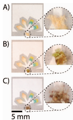
Figure 7. Devices run with 5 \mu\text{L} of contaminated samples of glucose and protein (4.5 mM glucose and 50 \mu\text{M} BSA). The solid contaminants (A) sawdust, (B) pollen, and (C) dirt are filtered from the samples and do not interfere with the assays, except in the case of the protein assay that is contaminated by the pollen.
