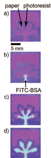
Figure 4. A 10 \mu\text{M} solution of FITC-BSA dissolved in 40 \text{ mM} phosphate buffer ( \text{pH} 7.4 ) was wicked into the paper-based device and imaged under UV light ( 254 \text{ nm} ). The FITC-BSA distributes evenly throughout the channels and test zones. (a) A device before wicking a solution containing FITC-BSA. (b) A device after wicking 1 \mu\text{L} of the FITC-BSA solution. (c) A device after wicking 2 \mu\text{L} of the FITC-BSA solution. (d) A device after wicking 5 \mu\text{L} of the FITC-BSA solution.
