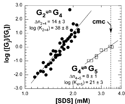
Figure 5. Plot of \log([G_j]/[G_i]) and \log([G_5]/[G_4]) vs \log [SDS] for four sets of experiments for the transition G _2 \rightarrow G _4 (●) and two sets for the transition G _4 \rightarrow G _5 (□), where [G _2 ], [G _4 ], and [G _5 ] are the relative concentrations of all UBI-SDS _n complexes within their respective groups. Values \Delta n_{i-j} correspond to the number of SDS molecules involved for the transition from G _i to G _j ( i and j represent the label of the group). For example, in the transition from G _2 to G _4 , the value \Delta n_{2-4} corresponds to the number of SDS that bind G _2 to yield G _4 , and K_{i-j} refers to the thermodynamic equilibrium constant for this transition ( K_{i-j} has units of (mol/L) ^{-\Delta n_{i-j}} ). Relative concentrations were determined by integrating electropherograms in the mobility range attributed to each group (integration was performed as a function of time, t ). We fitted the data to the linearized expressions of the law of mass action described in eqs 5 and 6. The errors ( \pm ) correspond to half of the amplitude between the highest and lowest values of the slope and y-intercept fitting the data points.
