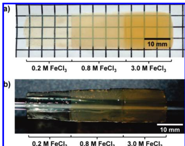
FIGURE 4. (a) Fe 3+ -AA film containing a step gradient in the concentration of the cross-linking ion, Fe 3+ . (b) Fe 3+ -AA film draped over a glass pipet to demonstrate the variable rigidity of the sections as a function of the concentration of Fe 3+ used to cross-link the AA. The section made from the least concentrated solution of Fe 3+ had the weakest mechanical rigidity. The labeled concentrations correspond to the solutions used to wet the region of the paper template that formed each section of the gel.
