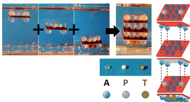
Fig. 5 The self-assembly of complex objects can be programmed by patterning the density of the levitating objects. Here, interlocking pieces were prepared by gluing polymer spheres to prepared 13 × 8 mm acrylic sheets (red). White layers are adhesive-backed Teflon. Each object is programmed to levitate at a different levitation height when placed in the same container together; after the objects self-aligned by placing the container in the magnetic field, the magnet-to-magnet distance was reduced from 60 mm to 30 mm to bring them into contact. The different spheres are: A – acrylic (PMMA), P – polystyrene and T – Torlon. The magnets were 3.5 × 2.5 × 1 in (89 × 64 × 25 mm).
