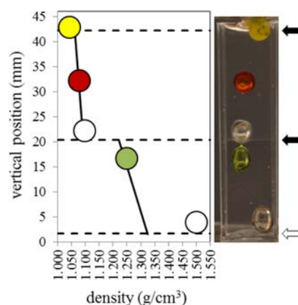
Figure 4. Preparing unequal gradients in density using an aqueous multiphase system (AMPS) formed from a paramagnetic salt as a medium for magnetic levitation (MagLev). A mixture of 16.7% (wt/vol) poly(ethylene glycol) and 875 mM MnSO 4 generates an AMPS with a large step in both density and magnetic susceptibility between phases. The gradients in density are illustrated by five density standard beads: 1.045 g/cm 3 (yellow), 1.081 g/cm 3 (red), 1.100 g/cm 3 (clear, middle), 1.250 g/cm 3 (green), and 1.500 g/cm 3 (clear, bottom). MagLev can be used to measure the densities of beads that levitate within a phase of the AMPS (red and green bead). We measure the height of each bead by calculating the centroid for each bead. Beads that contact a fluid interface (black arrows, air/liquid and liquid/liquid) rest at a height based on the combination of surface forces, magnetic forces, and gravitational forces. Beads at the solid/liquid interface (white arrow) at the bottom of the container rest on the inside surface of the container.
