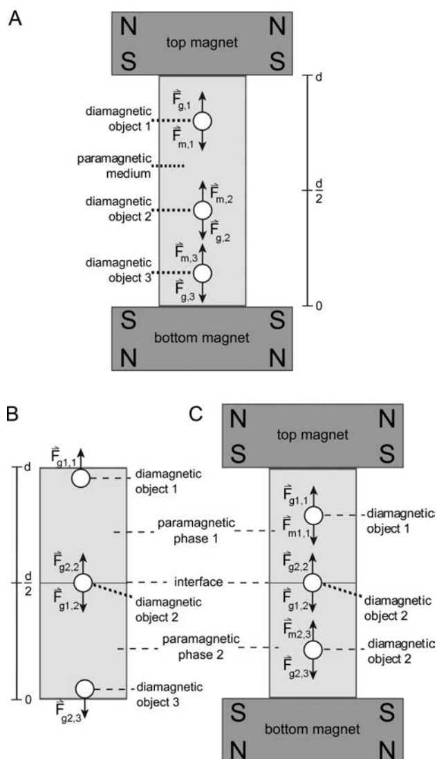
Figure 1. Schematic representations of the behavior of objects in magnetic levitation and in aqueous multiphase systems (AMPS). (A) Three diamagnetic objects levitate at different heights depending on the position at which the magnetic and gravitational forces ( F_m and F_g ) acting on the objects are in equilibrium. (B) In an AMPS, objects either float, sink, or come to rest at a liquid–liquid interface. (C) In a paramagnetic AMPS in a magnetic field gradient, a combination of behaviors is possible. Objects 1 and 3 levitate in the phases, while object 2 is trapped at the liquid–liquid interface. In this example, the interface between phases is located at the midpoint ( d/2 ) of the distance between the magnets.
