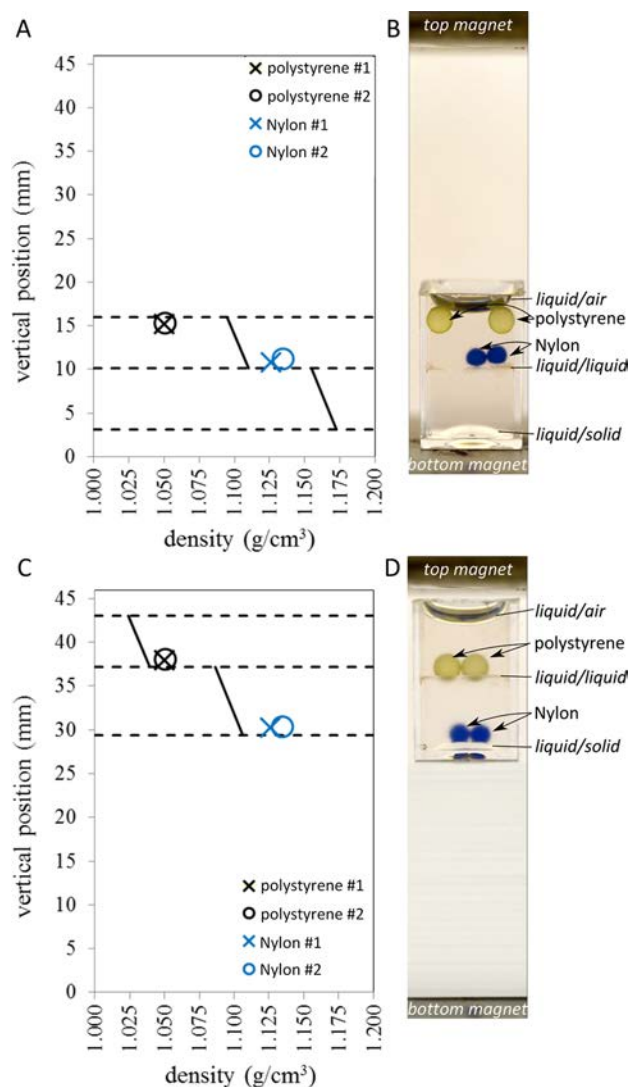
Figure 5. The step in density at the interface of a paramagnetic AMPS is dependent on the height of the interface in a MagLev device. When a small cuvette is at the bottom of the MagLev device, blue Nylon beads (blue “X” and circle) are binned at the liquid/liquid interface of the AMPS (A and B). When the cuvette is near the top of the MagLev device, white polystyrene beads (black “X” and circle) are captured at the liquid/liquid interface (C and D). Plots of the density versus position demonstrate illustrate the shift in the position of the gradient along the density axis (A and C). Dashed lines depict the liquid/air , liquid/liquid , and liquid/solid interfaces of an AMPS at the lower (A) and upper (C) positions. Images from experiments demonstrate the shift in the step in density by capturing Nylon beads in the lower position (B) and polystyrene beads in the upper position (D).
