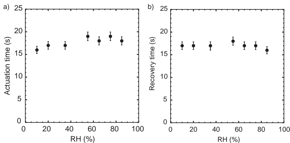
Figure 4. a) Actuation and b) recover times at different RH ( P = 1 W); in each case, the time is constant within \pm 10\% .
