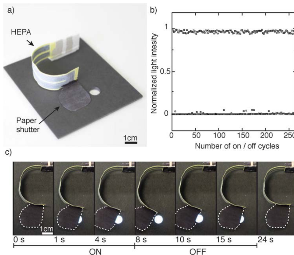
Figure 6. a) Photograph of a HEPA ( L:W = 5:1 cm) optical shutter ( P = 1 W; I = 1.5 mA; RH = 40\% ). b) Number of on/off cycles versus normalized light intensity calculated from the videos of actuation. c) Time-lapse photographs of the HEPA optical shutter. The device is placed on a backlit table, and the light is seen only when the shutter opens. The dashed lines highlight the shutter area.
