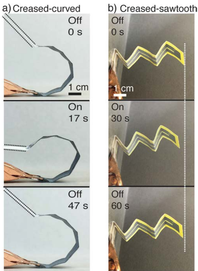
Figure 5. Time-lapse photographs of: a) creased-curved HEPA ( L:W = 7:0.8 cm): dashed lines highlight the attached passive paper; b) creased-sawtooth actuator fabricated with the tape positioned on alternating side of a HEPA ( L:W = 5:1 cm; P = 1 W; I = 1.5 mA; RH = 40\% ).
