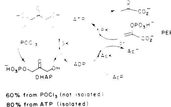
Scheme II. Chemical and Enzymatic Preparations of Dihydroxyacetone Phosphate
