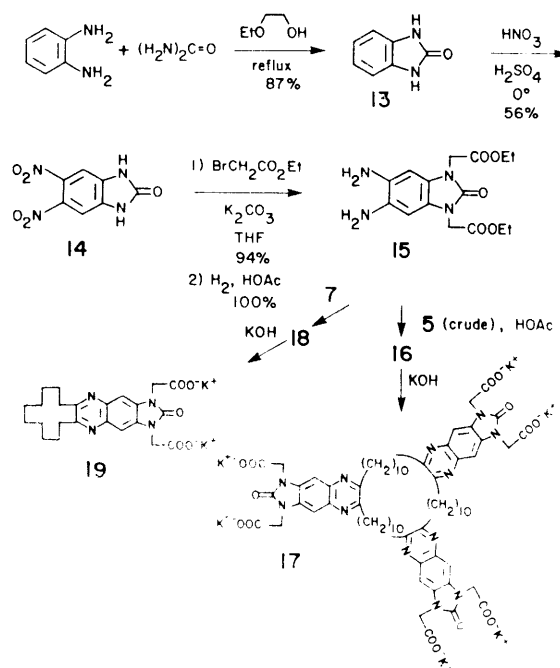
Scheme II. Synthesis of a Water-Soluble Macrocyclic Trisquinoxaline
