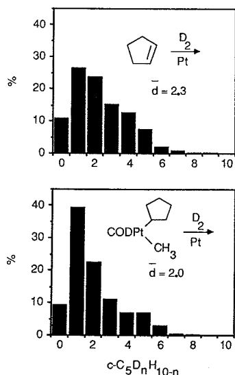
Figure 5. The isotopic composition of cyclopentanes from the deuteration ( -20\text{ }^{\circ}\text{C} , 2.3 atm) of (upper) cyclopentene and (lower) \text{CODPt}(\text{CH}_3)(\overline{\text{CH}}(\text{CH}_2)_3\text{CH}_2) .
