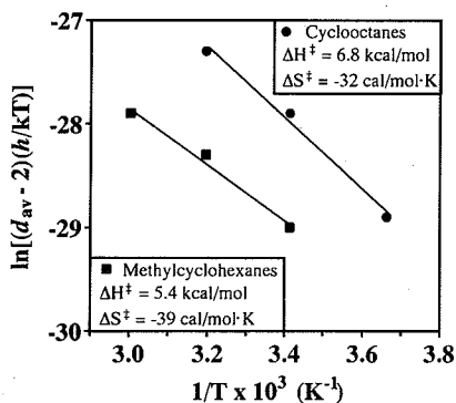
Figure 4. Plot of \ln[(d_{av} - 2)(h/kT)] vs 1/T for the reductions of cis -cyclooctene and 1-methylcyclohexene.
