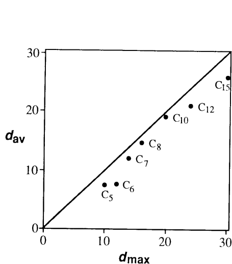
FIGURE 1. A plot of d_{\text{av}} vs d_{\text{max}} for the cycloalkanes produced in the heterogeneous reduction of unsubstituted cycloolefins using \text{H}_2 and \text{D}_2\text{O}/\text{THF} (1:1, v:v; \text{pD}(\text{D}_2\text{O}) = 1 ).
