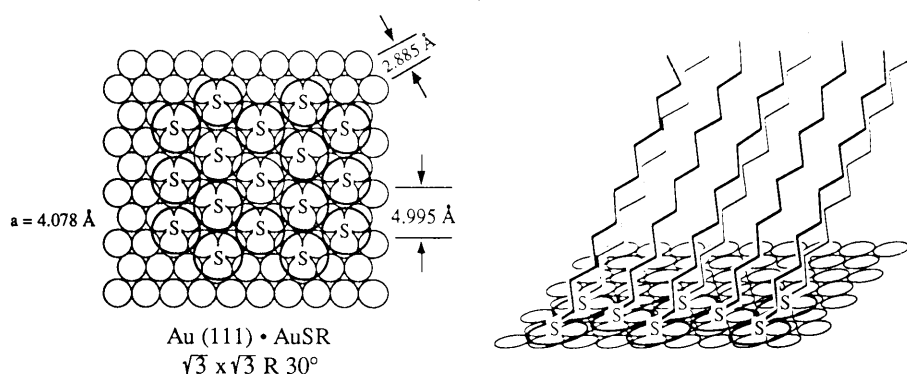
FIGURE 4. Structure of n -alkanethiolate monolayers formed on Au(111). The adsorbed alkanethiol forms an epitaxial layer on gold (left) generating a densely packed hydrocarbon layer that is canted \sim 30^\circ from the surface normal (right).
