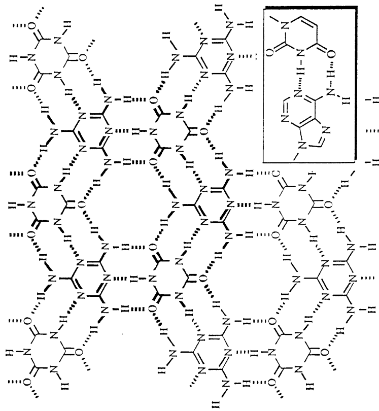
Figure 6. An idealized structure of the 1:1 complex between melamine and cyanuric acid (6-7). The inset shows the adenine-uracil base pair.
