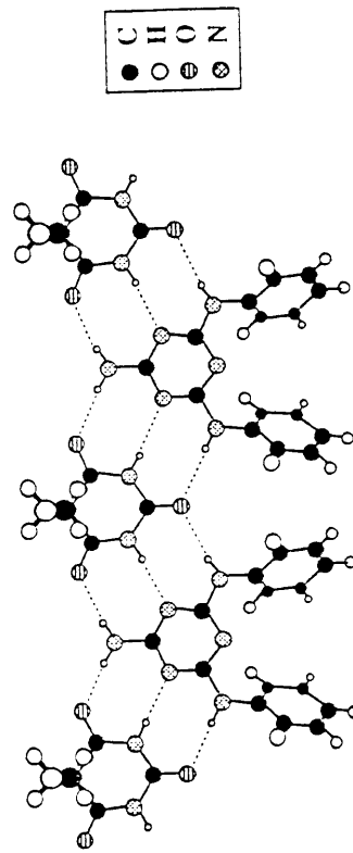
Figure 7. An X-ray crystal structure of the polymeric diphenyl melamine-diethyl barbituric acid (8-9) complex.
