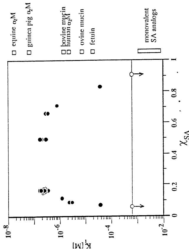
Figure 3. Inhibition of hemagglutination of erythrocytes by poly(2-co-acrylamide). (Reproduced from ref. 6. Copyright 1991 American Chemical Society.)
