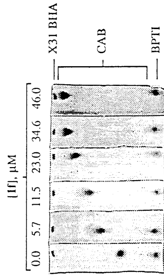
Figure 1. Affinity electrophoresis of bovine carbonic anhydrase B (CAB) on polyacrylamide slab gels containing various concentrations of affinity ligand 1f . Bovine pancreatic trypsin inhibitor (BPTI) and the bromelain-released hemagglutinin of influenza virus X-31 (X31 BHA) were used as internal standards.
