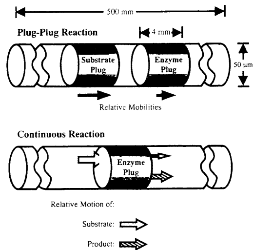
Figure 1. The substrate, of higher electrophoretic mobility than the enzyme, moves into the plug of enzyme and is consumed by enzyme-catalyzed reaction; the remaining unutilized substrate migrates away from this plug (the arrow exiting the plug in the continuous reaction format is narrowed to indicate reduction in concentration). A product (hatched arrow; continuous reaction format) that also has a higher electrophoretic mobility than that of the enzyme migrates from the enzyme-containing plug; in this instance its motion is in the same direction as that of the substrate leaving the plug. Different combinations of relative mobilities of the enzyme, substrates, and products will result in different combinations of relative directions of motion to and from the enzyme-containing region. The average mobility of the enzyme may also be modified on binding a charged substrate.
