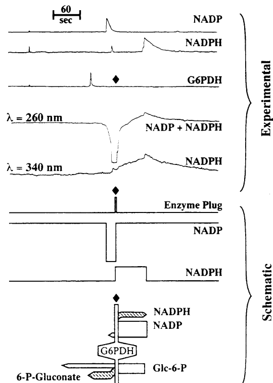
Figure 5. Oxidation of glc-6-P ( 200 \mu\text{M} ) using NADP ( 200 \mu\text{M} ). The full description of the figure is similar to Figure 3.
