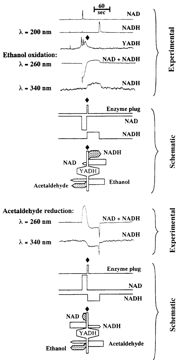
Figure 6. Yeast alcohol dehydrogenase-catalyzed oxidation of ethanol ( 200 \mu\text{M} ) using NAD ( 200 \mu\text{M} ) and reduction of acetaldehyde ( 200 \mu\text{M} ) using NADH ( 200 \mu\text{M} ). The full description of the figure is similar to Figure 3.
