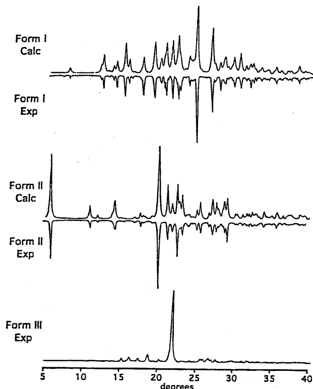
Figure 4. Comparison of experimental X-ray powder diffraction traces for three polymorphs of the X = Br complex with traces calculated from the solved crystal structures. There is no calculated trace for the third polymorph, since no single crystal suitable for X-ray diffraction could be grown.
