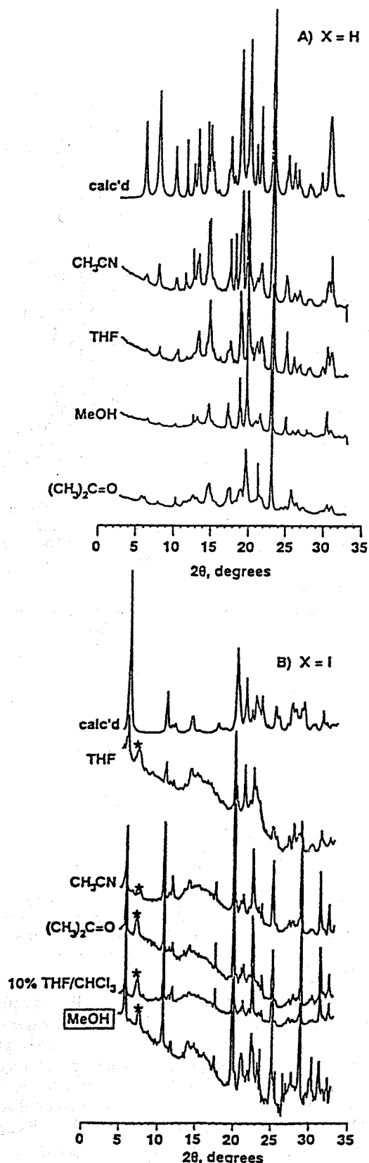
Figure 2. Experimental X-ray powder diffraction traces for X = H and I . Agreement with the calculated traces is only fair: although the peaks in the calculated trace are present in the observed traces, additional peaks are also observed and the agreement in intensities is poor. The boxed solvent is that used to grow the crystal studied by single-crystal diffraction (for X = H , the solvent for growth of single crystals was dichloromethane). The starred peak may be due to the sample holder or to a contaminant as in Figure 1.
