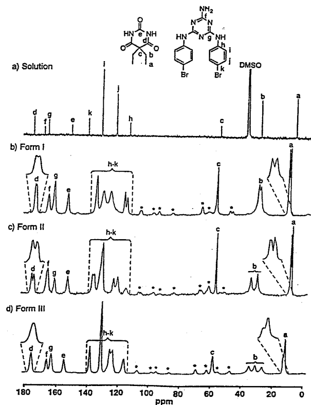
Figure 10. Solution and solid-state ^{13}\text{C} NMR spectra of X = \text{Br} polymorphs. Spinning sidebands are starred.
