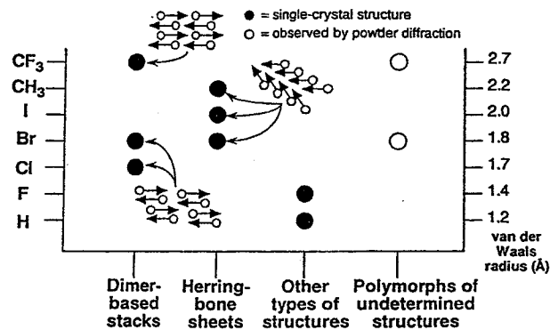
Figure 11. Relationship between the size of the substituent and the motif of tertiary crystalline architecture in complexes built from N,N' -bis( p - X -phenyl)melamines. Two varieties of dimer-based stacks and one of herringbone sheets are shown schematically. Arrows with circles attached represent end-on views of the tapes.
