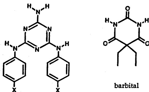
N,N' -bis( para -X-phenyl)melamine
