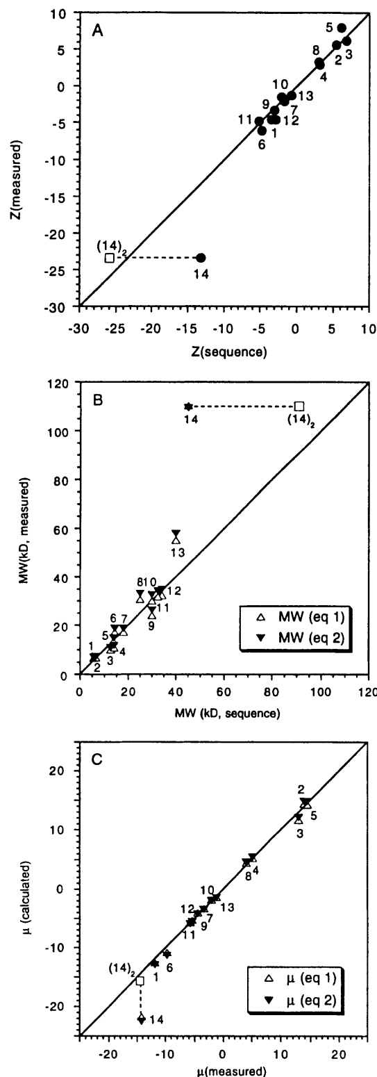
Figure 3. Comparison of values of effective charge (A) and molecular weight (B) of proteins from charge ladder experiments with those calculated based on amino acid sequences. (C) Comparison of electrophoretic mobility estimated using eq 1 or 2 with that determined from experiment. The open square in each figure indicates the theoretical values of Z_p(0) , molecular weight, and electrophoretic mobility for the dimer of ovalbumin. In all three figures, the scales for the x and y axes were the same, and a diagonal line was drawn to help the visual comparison.
