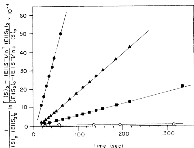
Figure 1. Rate constant plots for the reaction of several mono- and dithiols with Ellman's reagent in pH 7.0 phosphate buffer (0.05 M) at 30.0 \pm 0.5 °C under argon. The terms in the expression on the axis are defined as follows: for the monothiols, S_0 = [RS^-] + [RSH] , n = 1 ; for the dithiols, S_0 = [^-SRS^-] + [HSRS^-] + [HSRSH] , n = 2 (cf. eq 10 and 18 of the text). Reducing agents: ●, glycol dimercaptoacetate; ■, bis(2-mercaptoethyl) ether; ▲, N,N' -bis(2-mercaptoethyl)urea; ○, thioglycolic acid.
