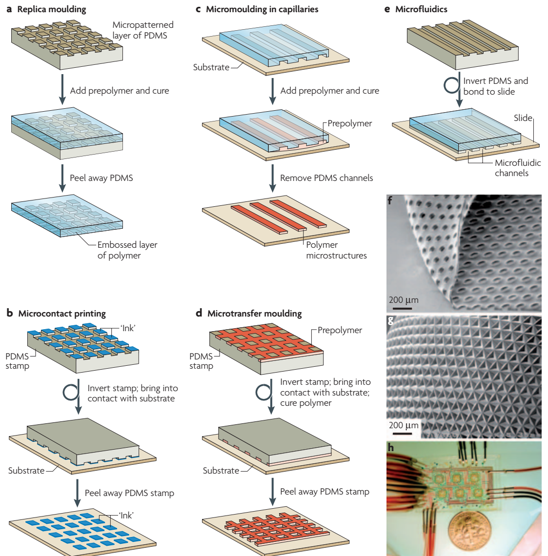
Figure 2 | The core techniques of soft lithography. The key stages of each of the following techniques are shown: a | replica moulding; b | microcontact printing; c | micromoulding in capillaries; d | microtransfer moulding; and e | microfluidics. f | A PDMS membrane with microfabricated holes created by replica moulding from a master with circular posts. g | A curved layer of micropatterned polyurethane created by bending a micropatterned layer of PDMS and then replica moulding against it. h | A microfluidic chemostat for the growth and culture of microbial cultures. The device incorporates six reactors with an intricate network of plumbing, in a footprint that is approximately 5 cm 2 . PDMS, poly(dimethylsiloxane). Part ( f ) reproduced with permission from REF. 74 © (2000) American Chemical Society. Part ( g ) reproduced with permission from REF. 1 © (1998) Gesellschaft Deutscher Chemiker. Part ( h ) reproduced with permission from REF. 59 © (2005) American Association for the Advancement of Science.
