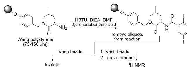
Figure 3. Schematic describing the process for monitoring conversion for a condensation reaction of a solid-supported amine with a carboxylic acid.
