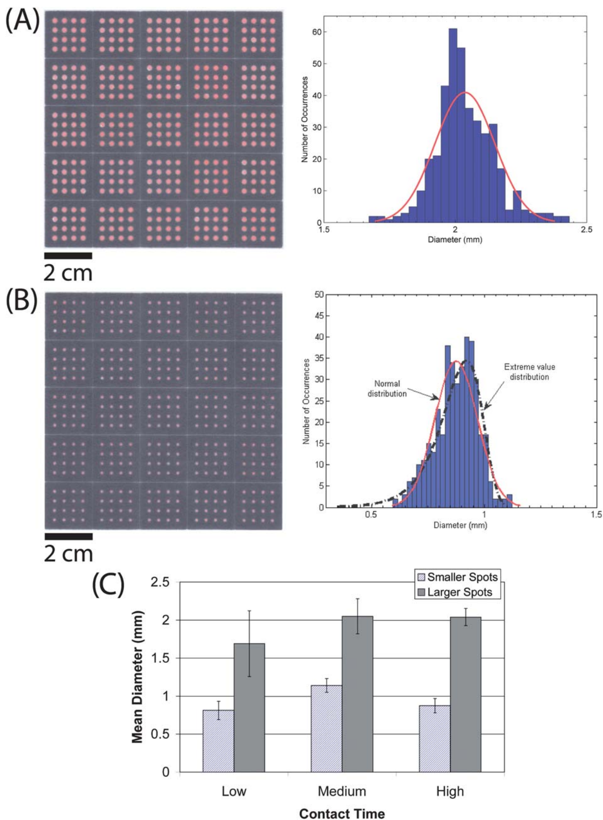
Fig. 3 Contact printing on pre-patterned Whatman Chromatography Paper No. 1. We used the technique of wax printing to pattern both the paper-based substrates receiving the water-soluble dye (Allura red) and the individual layers of patterned paper within the stamp. (A) Printed spots with a mean diameter of 2.0 \pm 0.1 mm with N = 400 (coefficient of variation of 5%) on a pre-patterned substrate. The accompanying histogram shows the distribution of the measured diameters, along with a fitted normal distribution. The contact time was 10 s. (B) Printed spots with a mean diameter of 0.9 \pm 0.1 mm
