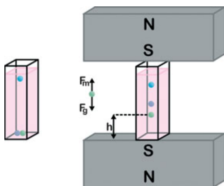
FIG. 1—Diamagnetic objects are placed in a paramagnetic solution, \text{MnCl}_2 in this work, and sink (purple and green spheres) or float (blue sphere) depending on the density of the object in comparison with that of the solution (left). The diamagnetic objects levitate, according to their density, when placed in a MagLev device that is composed of two magnets with like poles facing one another. The levitation height “ h ” of each object occurs when the gravitational force on the object ( F_g ) is canceled by the magnetic force ( F_m ) applied in the opposite direction.
