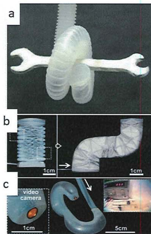
Figure 3. Examples of soft structures illustrating different functional modifications. a) A textured surface to improve gripping. Reproduced from Ref. [35b] with permission. Copyright 2013, John Wiley & Sons. b) A structure that includes an origami strain-limiting layer, with leaves glued together in specific points to control its bending. Reproduced from Ref. [33] with permission. Copyright 2012, John Wiley & Sons. c) A “tentacle” including a cell-phone camera and an optical link, with an image obtained with this system. Reproduced from Ref. [35b] with permission. Copyright 2013, John Wiley & Sons.
