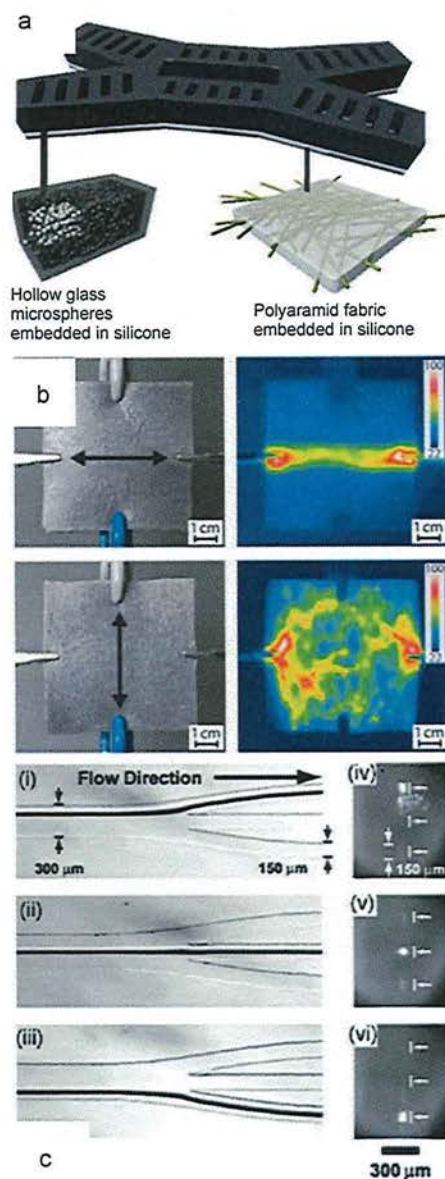
Figure 8. PDMS-based structures illustrating features that can be incorporated into soft robots. a) Glass microspheres (to decrease weight) and polyaramid fabric (for strength) in a walker (Figure 4). Reproduced from Ref. [36b] with permission Copyright 2014, Mary Ann Liebert, Inc. b) Anisotropic current flow (visualized in the IR as heat) in PDMS sheets containing steel wool on application of strain parallel (top) and perpendicular (bottom) to the orientation of the fiber, and the flow of current. [48] Reproduced from Ref. [48] with permission. Copyright 2015, John Wiley & Sons. c) Switchable fluidic optical light guide, [49] visualized with an optical microscope (i–ii) from the top of the microfluidic channels and (iv–vi) from the ends of the microfluidic channels. Reproduced from Ref. [49] with permission. Copyright (2004) National Academy of Sciences, U.S.A.
