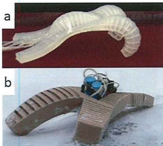
Figure 4. Quadruped “walkers” using five pneumatically controlled chambers: a) tethered to the pressure source through flexible tubes (length of walker \approx 20 cm); b) untethered, with compressor, valves, and other hard controllers riding on top of the soft walker (length \approx 0.5 m). Reproduced from Ref. [36b] with permission. Copyright 2014, Mary Ann Liebert, Inc.
