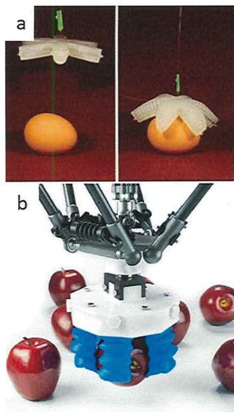
Figure 1. a) Soft gripper (a “starfish gripper”) picking up an uncooked egg. Reproduced from Ref. [32] with permission. Copyright 2011, John Wiley & Sons. b) An industrialized adaptation of a gripper. The “fingers” are soft and grip delicate objects (here, fruit) without damage. The “palm” of the gripper is hard and attached to a commercial, hard, arm. (Soft Robotics, Inc.). Both rely on PneuNets and pneumatic actuation.
