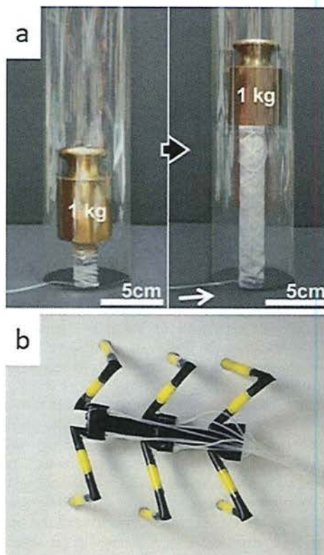
Figure 7. a) A PDMS tube, reinforced with a paper origami strain-limiting structure, lifts a heavy weight on pressurization. Reproduced from Ref. [33] with permission. Copyright 2012, John Wiley & Sons. b) An arthrobot, in which the combination of flexible but non-elastic tubes (polypropylene drinking straws) and PDMS balloons (inside these tubes) provides a joint that mimics functional aspects of the joints of a spider.
