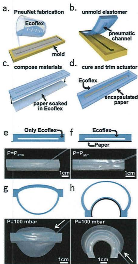
Figure 2. a–d) Schematic of techniques used to mold and assemble a PDMS/paper composite. e–h) Cross-sections of PDMS (“Ecoflex”) structures, both with and without a paper strain-limiting layer, (uninflated and inflated), together with photographs of these structures inflated and uninflated. Reproduced from Ref. [33] with permission. Copyright 2012, John Wiley & Sons.
