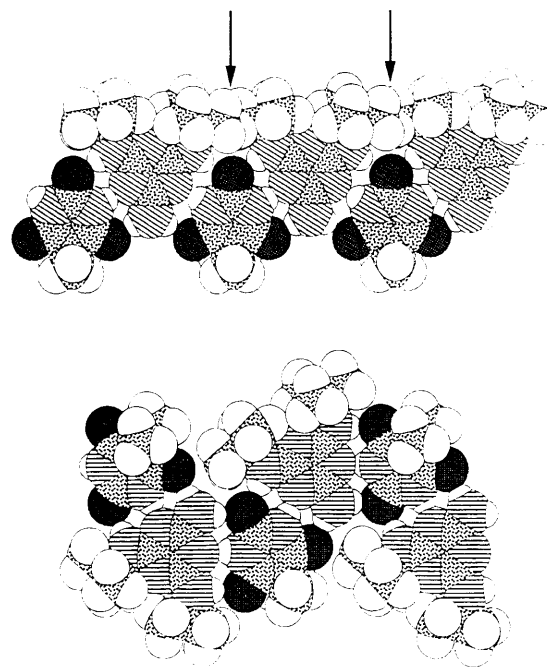
Figure 1. Top: Hypothetical linear tape of the Mel( t Bu) 2 ·Bar(CH 3 ) 2 complex, with regions of steric repulsion indicated by arrows. Bottom: The observed crinkled format of this complex, which relieves the steric hindrance.
