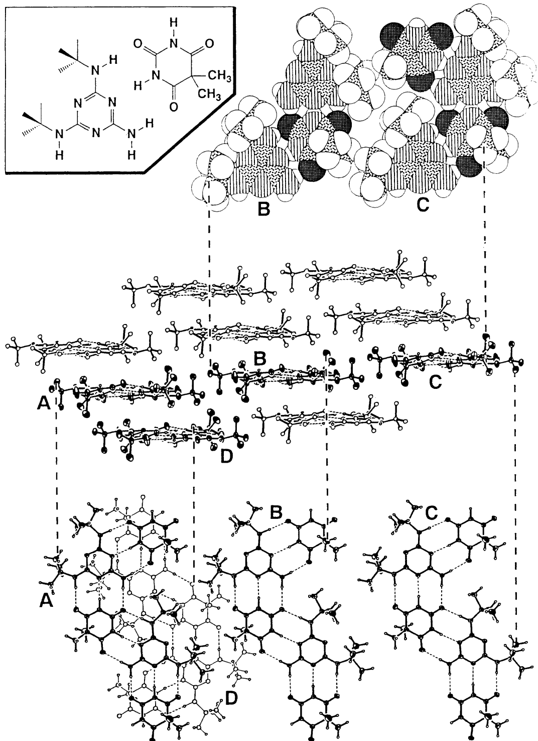
Figure 5. Views of the Mel( t Bu) 2 -Bar(CH 3 ) 2 complex. Alkyl hydrogens have been omitted from the central view.
