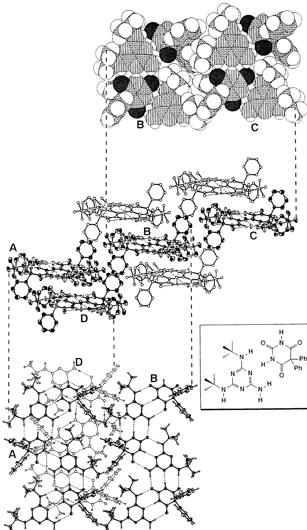
Figure 6. Views of the \text{Mel}(\text{tBu})_2\text{-Bar}(\text{Ph})_2 complex. Alkyl and aryl hydrogens have been omitted from the central view.
