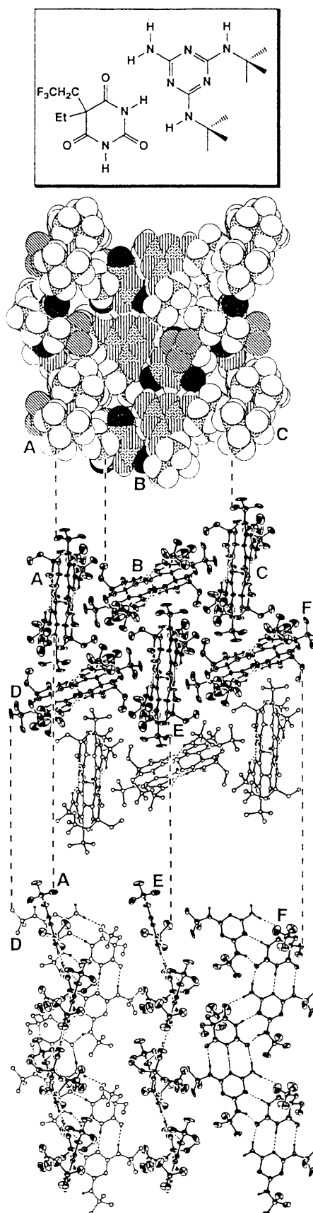
Figure 4. Views of the Mel('Bu) 2 -Bar(Et)(CH 2 CF 3 ) complex. Alkyl hydrogens have been omitted from the central and bottom views.
