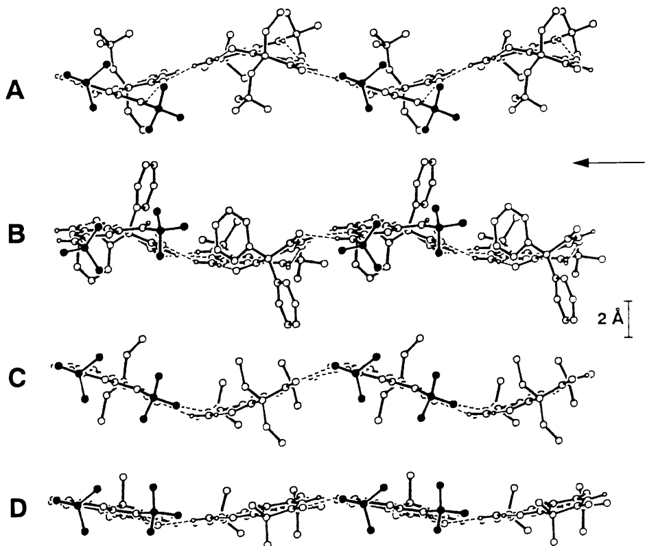
Figure 2. Side views of crinkled tapes of Mel( t Bu) 2 complexes showing their deviation from planarity: (A) Bar(Et)(CH 2 CF 3 ) complex; (B) Bar(Ph) 2 complex; (C) Bar(Et) 2 complex; (D) Bar(CH 3 ) 2 complex. The deviation decreases from A to D (see Table 1). The arrow indicates the direction of a view down the long tape axes. The filled-in tert -butyl groups are on the edges of the tapes that are nearer to the viewer.
