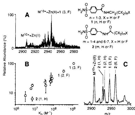
Figure 1. (A) Mass spectra of the 10+ charge state of BCAII (1.0 \mu M) and 18 inhibitors (0.05 \mu M each) in 10 mM \text{NH}_4\text{OAc} (pH 7.0). (B) Correlation of the relative ion abundances with the values of K_b in solution. Six of the K_b values represent the sum of those from two inhibitors with the same mass. The relative errors of solution K_b measurements were 20–30%. (C) Mass spectra of BCAII (1.0 \mu M) and four inhibitors (2 (1, H) = 60 \mu M, 1 (2, H) = 3.0 \mu M, 2 (6, F) = 1.5 \mu M, 1 (3, F) = 0.1 \mu M) in 10 mM \text{NH}_4\text{OAc} (pH 7.0).
