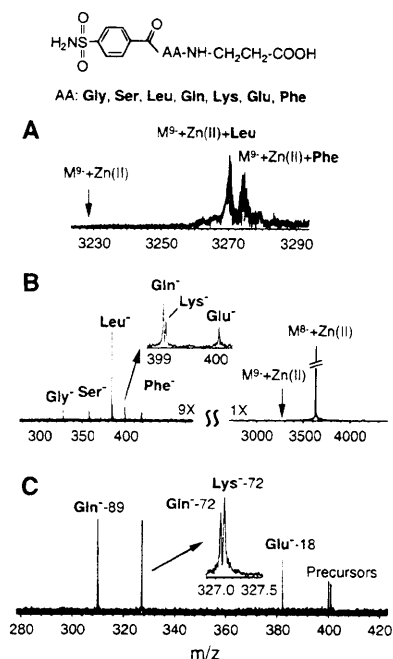
Figure 2. Negative ESI-FTICR mass spectra of BCAII (7.0 \mu M) with inhibitors (7.0 \mu M each) in 10 mM NH_4OAc (pH 7.0). The multistep dissociation experiments include the following. (A) Mass spectra of complex ions of BCAII with inhibitors (9- charge state) before ion isolation. (B) Isolation of 9- complex ion species using m/z -selective ion accumulation and subsequent dissociation of the complexes with 0.5-s rf irradiation ( V_{pp} = 12 V, collision gas nitrogen \sim 10^{-7} Torr). The intensity of the dissociated inhibitors correlates with their binding affinity. The arrow points to the m/z of the precursor that has been completely dissociated. (C) SWIFT isolation and dissociation of three of the inhibitor ions (from B), Glu^- , Lys^- , and Gln^- at m/z 399-401 (0.5-s rf irradiation with V_{pp} = 12 V and collision gas nitrogen \sim 10^{-7} Torr). The precursor ions were attenuated 95%. New peaks result from the fragmentation of the inhibitors.
