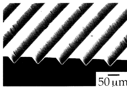
FIG. 2. Scanning electron micrograph of a contoured film of polyurethane supported on a glass slide (as in Fig. 1, part g). The contoured substrate was frozen in nitrogen, fractured along a plane perpendicular to the array of lines, and sputtered with gold (20 nm) prior to the electron microscopy.
