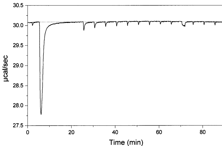
Figure 7. ITC titration of R_tV_3 by R'_tL'_3 (0.126 mM) in 5.0 mM phosphate buffer at 298 K. The injected volumes of the first, second, and twelfth injections were 0.5, 35, and 35 \mu\text{L} , respectively, and 3.0 \mu\text{L} for the remaining injections. The interval between the second and third injections was 20 min; the interval between the remaining injections was 5 min.
