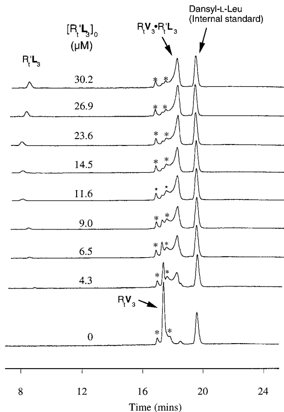
Figure 4. HPLC chromatograms of the titrated solution of R_1V_3 ( 4.5 \mu\text{M} ) on addition of aliquots of R_1L'_3 ( 1.06 \text{ mM} ) solution in the presence of L ( 19.1 \text{ mM} ). The sample of R_1V_3 used here contained small amounts of impurities, which are indicated by the symbols (*). The HPLC conditions were similar to those described in Figure 3, except that a Vydac analytical RP column was used with the same linear gradient, run over 30 min.
