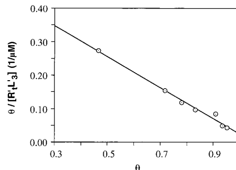
Figure 5. A plot of the ratios of \theta/[R_1L'_3] versus \theta for the titration of R_1V_3 ( 4.5 \mu\text{M} ) with R_1L'_3 ( 0\text{--}35 \mu\text{M} ) in the presence of L ( 19.1 \text{ mM} ). The line is a linear fit of the data to eq 13. The slope of the line yields a value of K/[L]^3 \approx 0.47 \mu\text{M}^{-1} . The value of K_d^t for R_1V_3 \cdot R_1L'_3 is thus estimated as \sim 4 \times 10^{-17} \text{ M} (an average value of three repetitions; the error is within 25%).
