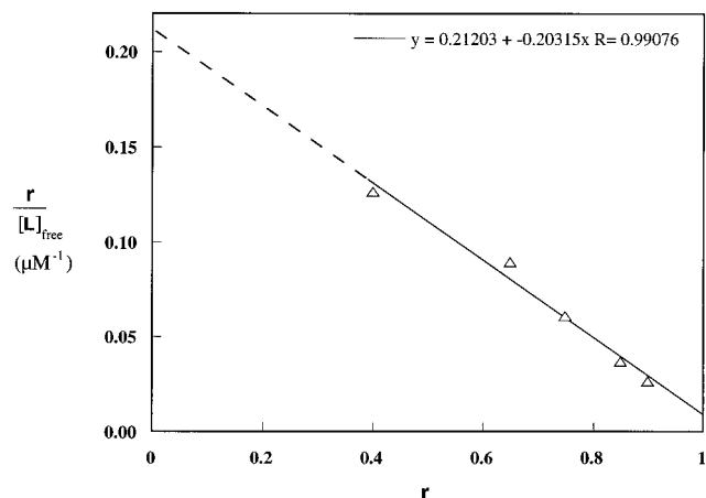
Figure 2. UV difference spectroscopy at 280 nm to determine K_d of L to R_1V_3 at pH 7.0 in the 20 mM phosphate buffer. R_1V_3 (2.1 \mu M, 3.0 mL) in a 1-cm cell was titrated against a solution of L (8.5 mM). The fraction function r was defined as the ratio of the change in the absorbance at 280 nm to the maximal change ( r = \Delta A^{280}/\Delta A_{max}^{280} ).
