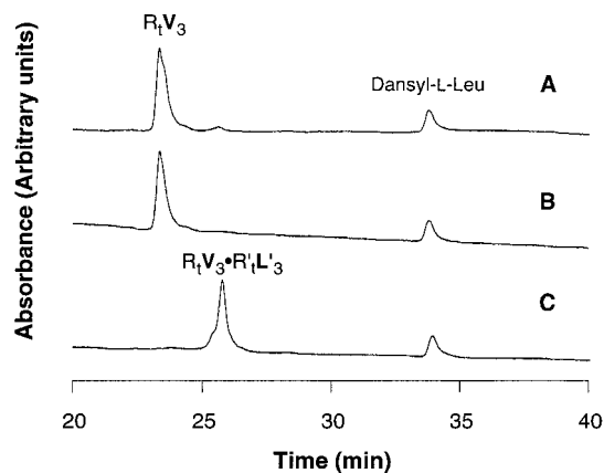
Figure 3. HPLC of aliquots of samples that contained (A) R_1V_3 ( 4.5 \mu\text{M} ), (B) R_1V_3 ( 4.5 \mu\text{M} ) + L ( 19.1 \text{ mM} ), and (C) R_1V_3 ( 4.5 \mu\text{M} ) + R'_1L'_3 ( 4.5 \mu\text{M} ). Dansyl-L-leucine ( 10 \mu\text{M} ) was introduced into each sample as an internal standard. All analyses were carried out under the same conditions: Rainin analytical reverse-phase (RP) C_{18} column, linear elution gradient from 85% solvent A [0.1% trifluoroacetic acid (TFA) in water] and 15% solvent B (0.1% TFA in acetonitrile) to 70% A and 30% B, over 45 min. The absorbance was monitored at 280 nm.
