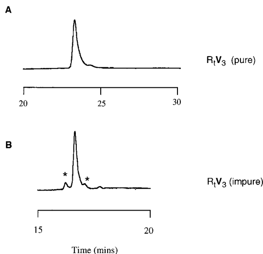
Figure 1. HPLC chromatograms of R_1V_3 . (A) Pure R_1V_3 and (B) R_1V_3 containing about 10% impurities marked by asterisk signs (*).
