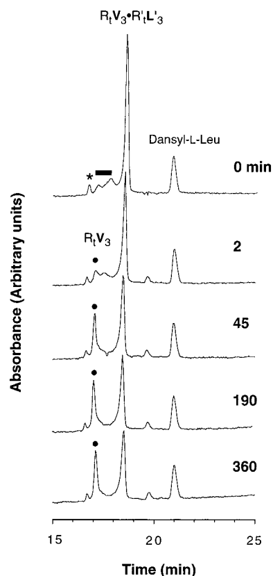
Figure 6. Representative HPLC traces demonstrating the exchange of R_1V_3 ( 3 \mu\text{M} ) + R_1L'_3 ( 22 \mu\text{M} ) with L ( 86 \text{ mM} ) with formation of R_1V_3 \cdot 3L . Exchange reactions were carried out by adding L to an equilibrated mixture of R_1V_3 and R_1L'_3 , and injecting the resulting mixture into the HPLC column after 0, 2, 45, 190, or 360 min. Symbols (•) indicate the retention time of R_1V_3 \cdot 3L ; this compound dissociates to free R_1V_3 on the column. The sample of R_1V_3 used here contained small amounts of impurities, which are indicated by the symbols (* and ■). The conditions were similar to those in Figure 3, except that a Vydac analytical RP column was used with the same linear gradient, run over 30 min.
