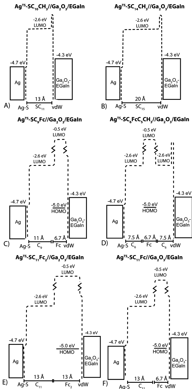
Figure 7. Energy level diagrams at open circuit for the \text{Ag}^{\text{TS}}\text{-SC}_{10}\text{CH}_3/\text{Ga}_2\text{O}_3/\text{EGaIn} (A), \text{Ag}^{\text{TS}}\text{-SC}_{14}\text{CH}_3/\text{Ga}_2\text{O}_3/\text{EGaIn} (B), \text{Ag}^{\text{TS}}\text{-SC}_9\text{Fc}/\text{Ga}_2\text{O}_3/\text{EGaIn} (C), \text{Ag}^{\text{TS}}\text{-SC}_6\text{FcC}_5\text{CH}_3/\text{Ga}_2\text{O}_3/\text{EGaIn} (D), \text{Ag}^{\text{TS}}\text{-SC}_{11}\text{Fc}_2/\text{Ga}_2\text{O}_3/\text{EGaIn} (E), and \text{Ag}^{\text{TS}}\text{-SC}_{11}\text{Fc}/\text{Ga}_2\text{O}_3/\text{EGaIn} (F) junctions. Dashed lines indicate the width and height of the barriers. The barrier presented by the alkyl chain has a barrier height, defined by the LUMO of the alkyl chain, of -2.6 \text{ eV} and a barrier width, defined by the length of the alkyl chain, of 1.3 \text{ nm} . The HOMO levels of the Fc and \text{Fc}_2 were estimated from the cyclic voltammograms (see text), and the LUMO level is approximately -0.4 \text{ eV} . 68,69 The width of the HOMO level of the \text{Fc}_2 is approximately twice that of the HOMO level of the Fc. The barrier width and height of the van der Waals interface (vdW) are not known and are discussed in more detail in the text. Ag-S represents the silver-thiolate bond; \text{C}_9 , \text{C}_{11} , \text{C}_{15} , and \text{C}_6 are alkyl chains; and Fc is ferrocene.
