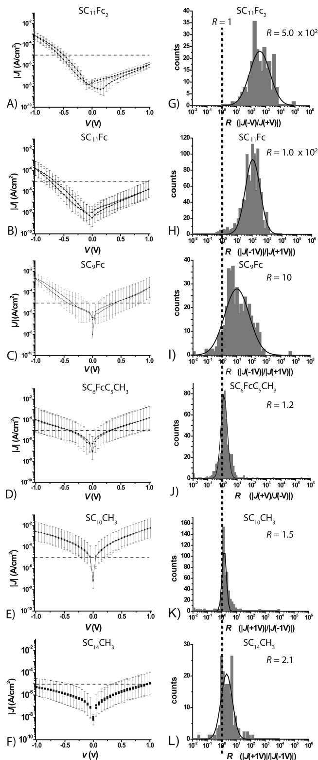
Figure 6. Average I/V curves of the \text{Ag}^{\text{TS}}\text{-SC}_{11}\text{Fc}_2/\text{Ga}_2\text{O}_3/\text{EGaIn} (A), \text{Ag}^{\text{TS}}\text{-SC}_{11}\text{Fc}/\text{Ga}_2\text{O}_3/\text{EGaIn} (B), \text{Ag}^{\text{TS}}\text{-SC}_9\text{Fc}/\text{Ga}_2\text{O}_3/\text{EGaIn} (C), \text{Ag}^{\text{TS}}\text{-SC}_6\text{FcC}_5\text{CH}_3/\text{Ga}_2\text{O}_3/\text{EGaIn} (D), \text{Ag}^{\text{TS}}\text{-SC}_{10}\text{CH}_3/\text{Ga}_2\text{O}_3/\text{EGaIn} (E), and \text{Ag}^{\text{TS}}\text{-SC}_{14}\text{CH}_3/\text{Ga}_2\text{O}_3/\text{EGaIn} (F) junctions. The error bars are defined by the log-standard deviation, as in Figure 5 (see text). The dashed line is a guide for the eye placed at J = 10^{-5} \text{ A/cm}^2 . The histograms of the rectification ratios R = |I(-V)/I(+V)| at \pm 1 \text{ V} are shown with Gaussian fits to these histograms for the \text{Ag}^{\text{TS}}\text{-SC}_{11}\text{Fc}/\text{Ga}_2\text{O}_3/\text{EGaIn} (G), \text{Ag}^{\text{TS}}\text{-SC}_{11}\text{Fc}_2/\text{Ga}_2\text{O}_3/\text{EGaIn} (H), and \text{Ag}^{\text{TS}}\text{-SC}_9\text{Fc}/\text{Ga}_2\text{O}_3/\text{EGaIn} (I) junctions. The histograms of the rectification ratios R = |I(V)/I(-V)| at \pm 1 \text{ V} are shown with Gaussian fits to these histograms for the \text{Ag}^{\text{TS}}\text{-SC}_6\text{FcC}_5\text{CH}_3/\text{Ga}_2\text{O}_3/\text{EGaIn} (J), \text{Ag}^{\text{TS}}\text{-SC}_{10}\text{CH}_3/\text{Ga}_2\text{O}_3/\text{EGaIn} (K), and \text{Ag}^{\text{TS}}\text{-SC}_{14}\text{CH}_3/\text{Ga}_2\text{O}_3/\text{EGaIn} (L) junctions. The dashed line is a guide for the eye placed at R = 1 .
