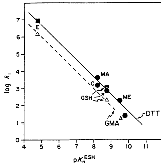
Figure 5. Rates of reduction k ( \text{M}^{-1} \text{min}^{-1} ) of symmetrical disulfides ESSE by thiolate anion, using dithiothreitol (DTT) or glycol dimercaptoacetate (GMA) as reducing agent. The lines have slope -1.0 . Data for reduction using DTT are indicated by filled symbols, and are taken from this paper or ref 12 ( \blacksquare ) or from Creighton ( \bullet ); 22 data for reductions using GMA are indicated by \Delta . The disulfides are identified by abbreviations for the corresponding thiols: E, Ellman's anion; MA, 2-mercaptoethylamine; C, cysteine; GSH, glutathione; ME, 2-mercaptoethanol; A, mercaptoacetic acid.
