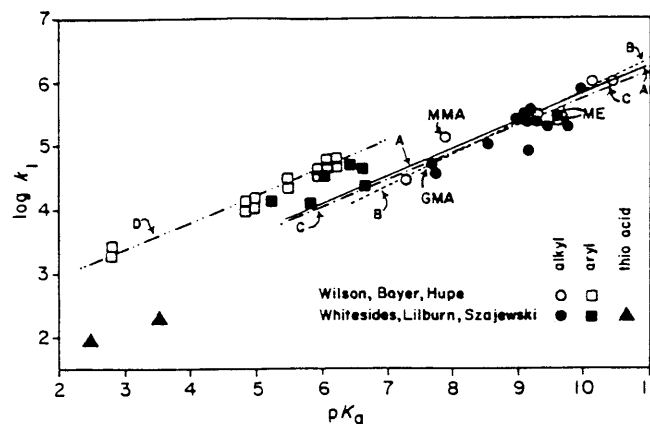
Figure 4. Collected rate constants ( \text{M}^{-1} \text{s}^{-1} ) for reduction of Ellman's reagent by thiols. Data from ref 12 are represented by solid points; data from ref 13 are represented by open points. Data for alkyl thiols are summarized by \bullet and \circ ; data for aryl thiols by \blacksquare and \square ; data for thiol acids by \blacktriangle . ME is mercaptoethanol; GMA is glycol dimercaptoacetate; MMA is methyl mercaptoacetate. Other points are identified in ref 12 and 13. The lines represent least-squares fits to these sets of data: A (—), alkyls ( \circ ), \beta_{\text{nuc}} = 0.43 , r^2 = 0.91 ; B (---), alkyls ( \circ ) 13 excluding methyl mercaptoacetate, \beta_{\text{nuc}} = 0.49 , r^2 = 0.97 ; C (-.-.-), alkyls ( \bullet ), \beta_{\text{nuc}} = 0.41 , r^2 = 0.67 ; D (- - - -), aryls ( \square ), \beta_{\text{nuc}} = 0.44 , r^2 = 0.97 .
