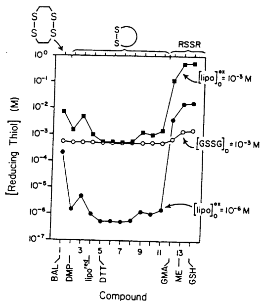
Figure 11. Concentrations of thiols required to reduce by half the concentration of the indicated disulfide group in solutions originally containing oxidized lipamide ( 10^{-3} M, \blacksquare ), oxidized glutathione ( 10^{-3} M, \circ ), and oxidized lipamide ( 10^{-6} M, \blacktriangle ). Compound numbers refer to Table V. The schematic structures at the top of the figure represent the type of disulfide believed to be formed from the thiol reducing agent (cyclic dimeric, cyclic monomeric, and intermolecular, respectively).
