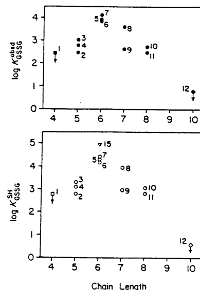
Figure 9. Plots of \log K_{\text{GSSG}}^{\text{obsd}} and \log K_{\text{GSSG}}^{\text{SH}} vs. chain length for the reduction of oxidized glutathione (GSSG) by a series of dithiols at 30.0 \pm 0.5^\circ\text{C} in pH 7.0 phosphate buffer under argon. The numbers refer to Table V. All dithiols are believed to form cyclic disulfides on oxidation, with the exception of 2,3-dimercaptoethanol (□, ■, 1), which may form a cyclic dimer (see the text), and glycol dimeracetoacetate (◇, ◆, 12), which forms a linear polymer. The point for the dithioketopiperazine (▽, 15) was obtained in an organic solvent. The units of K_{\text{GSSG}}^{\text{obsd}} and K_{\text{GSSG}}^{\text{SH}} are M. The equilibrium constants for these dithiols cannot be contrasted directly for that with monothiols, since the units are different. For comparison, however, addition of a small quantity of GSSG to a 1 M solution of 2-mercaptoethanol, a 0.22 M solution of glycol dimeracetoacetate, and a 1.4 \times 10^{-4} \text{ M} solution of DTT would produce the same ratio of (\text{GSH})/(\text{GSSG}) .
