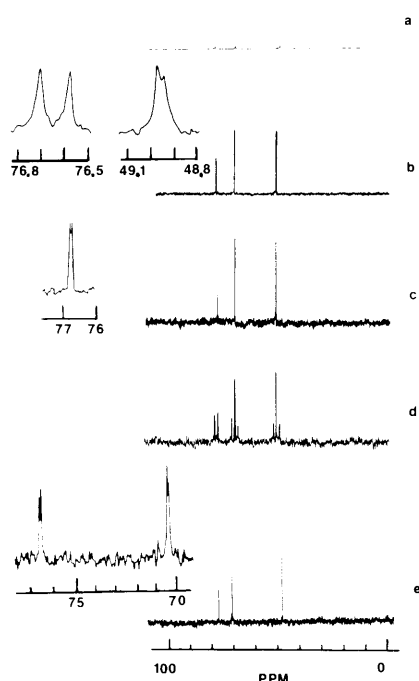
Figure 3. Proton-decoupled ^{13}\text{C} NMR spectra of D-3-aminopropane-1,2-diol-3-phosphate and related species: (a) DL-3-aminopropane-1,2-diol, (b) D-3-aminopropane-1,2-diol-3-phosphate prepared by phosphorylation catalyzed by glycerol kinase, (c) DL-3-aminopropane-1,2-diol-1-phosphate prepared chemically (eq 4), (d) off-resonance decoupled spectrum of (b), (e) L-3-aminopropane-1,2-diol-1-phosphate prepared chemically (eq 5).
