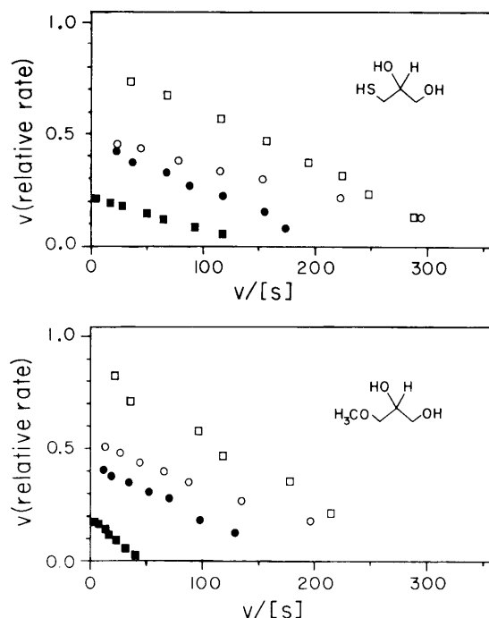
Figure 6. Eadie-Hofstee plots for phosphorylation of DL-3-mercapto-propane-1,2-diol (upper) and DL-3-methoxypropane-1,2-diol (lower) catalyzed by glycerol kinase. The sources of the glycerol kinase used in these experiments were from C. mycoderma (●), S. cerevisiae (■), B. stearotherophilus (●), and E. coli (□).
