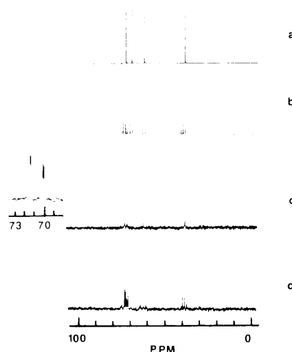
Figure 5. Proton-decoupled ^{13}\text{C} NMR spectra of D-butane-1,2,4-triol-1-phosphate and related species: (a) DL-butane-1,2,4-triol, (b) off-resonance spectrum of (a), (c) D-butane-1,2,4-triol-1-phosphate prepared by phosphorylation catalyzed by glycerol kinase, (d) off-resonance decoupled spectrum of (c).
