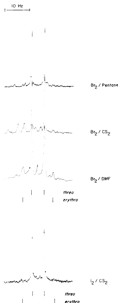
Figure 2. Deuterium-decoupled 100-MHz nmr spectra of the CHDBr resonances of (\text{CH}_3)_3\text{CCHDCHBr} obtained by bromination of erythro - 2 in pentane and \text{CS}_2 , the (\text{CH}_3)_3\text{CCHD} resonances from its bromination in DMF, and the CHDI proton from its iodination in \text{CS}_2 .
