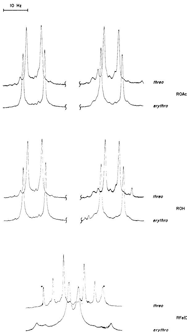
Figure 1. Deuterium-decoupled 100-MHz nmr spectra of the CHDCHD protons of threo - and erythro -(CH 3 ) 3 CCHDCHDOAc, -(CH 3 ) 3 CCHDCHDOH (1), and -(CH 3 ) 3 CCHDCHDFe(CO) 2 Cp (2). The peaks marked with asterisks in the spectrum of 2 are due to impurities.
