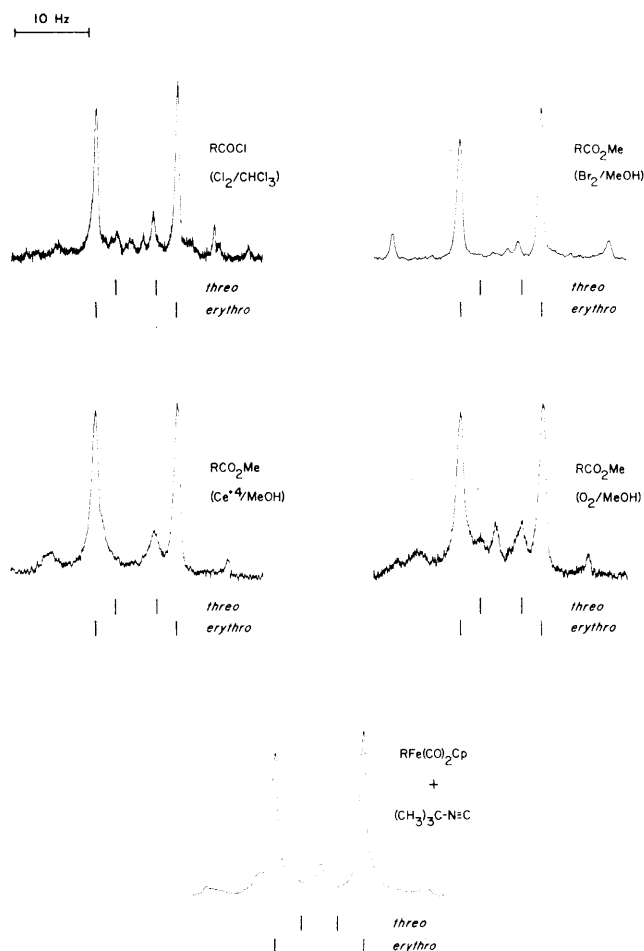
Figure 3. Deuterium-decoupled 100-MHz nmr spectra of products resulting from carbonyl insertion reactions of erythro -2.
