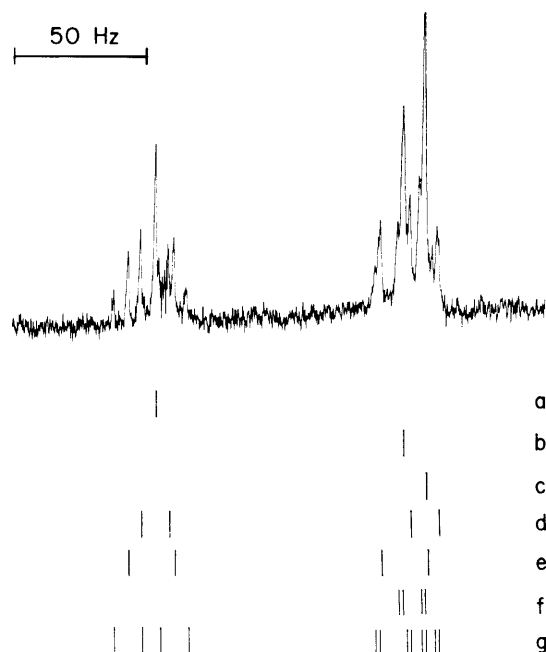
Figure 6. Deuterium-decoupled 100-MHz nmr spectra of the mixture of olefins obtained by thermal decomposition of erythro -2. The stick spectra under the experimental spectrum represent the positions of the various deuterated olefins, based on coupling constants of 1.6 Hz (geminal), 10.6 Hz (cis), and 17.4 Hz (trans); where indicated, Z and E designate the configuration of the substance around the olefinic bond: a, 1,1-d 2 , 3,3-dimethylbut-1-ene- 1,1-d 2 ; b, -E-1,2-d 2 ; c, -Z-1,2-d 2 ; d, -Z-1-d 1 ; e, E-1-d 1 ; f, -2-d 1 ; g, -d 0 . The chemical shifts used for these spectra varied slightly between compounds as a result of isotope effects, but (approximately) \nu_1 \sim 5.81 \delta , \nu_2 = 4.80 \delta , and \nu_3 = 4.88 \delta .
