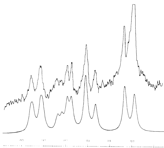
Figure 7. Deuterium-decoupled 100-MHz nmr spectrum of the CHDCHD protons of threo -( \text{CH}_3 ) 3 CCHDCHDFe(CO)(PPh 3 )Cp. For comparison, the computer simulated spectrum is given below the observed trace. The large peak at ca. 0.98 ppm is due to an impurity.
