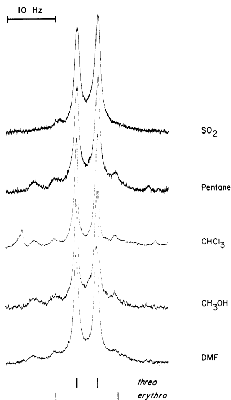
Figure 4. Deuterium-decoupled 100-MHz nmr spectra of the \text{CHDSO}_2 protons of (\text{CH}_3)_3\text{CCHDCHDSO}_2\text{Fe}(\text{CO})_2\text{Cp} produced by reaction of erythro -2 with sulfur dioxide in a variety of solvents. The approximate concentrations of \text{SO}_2 in each solvent (v/v) are: \text{SO}_2 (100); pentane (10); \text{CHCl}_3 (10); \text{CH}_3\text{OH} (10); DMF (10).
