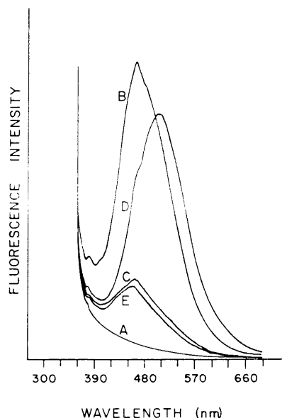
Figure 5. The fluorescence of PE-CONHNH-DANS is quenched by 1 N aqueous HCl: A, PE-CO 2 H; B, PE-CONHNH-DANS, dry film; C, PE-H (dry film) carried through the procedure to prepare PE-CONHNH-DANS from PE-CONHNH 2 (the fluorescence is due to adsorbed dansyl moieties); D, PE-CONHNH-DANS in contact with water for 1 h; E, PE-CONHNH-DANS in contact with 1 N HCl. Instrumental settings were identical for all spectra.
