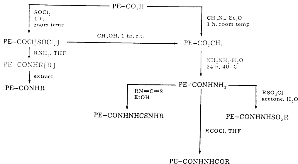
Scheme 1. Procedures Used to Couple Organic Groups to PE-CO 2 H. In This Scheme, "Extract" Indicates That the Film Is Treated for 18 h in a Soxhlet Apparatus with 2-Propanol (72–76 °C in extraction thimble)
