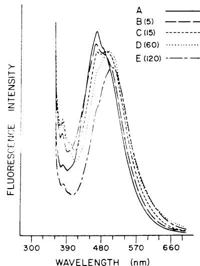
Figure 6. The wavelength of the fluorescence maximum of PE-CONHNH-DANS shows a time-dependent shift on contact with water: A, PE-CONHNH-DANS, dry film; B-E, PE-CONHNH-DANS, in contact with water for the indicated time (min). The instrument gain was adjusted to obtain spectra of equivalent intensity.
